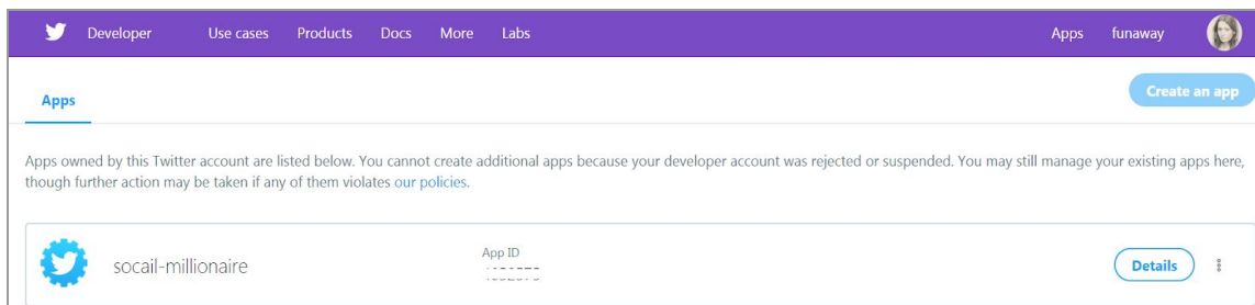
Fig. 8: Apps Page
