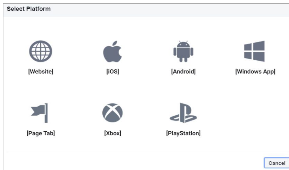
Fig. 11: 'Select Platform'
