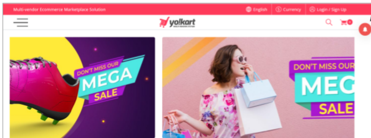
Fig. 2: Website Front-end
