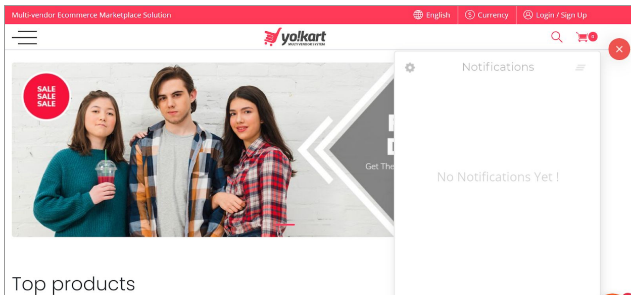
Fig. 2: Notifications Section
